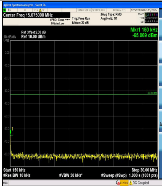
Band2-3MHz-QPSK-19185-1RB#0-1000~3000-P ASS
