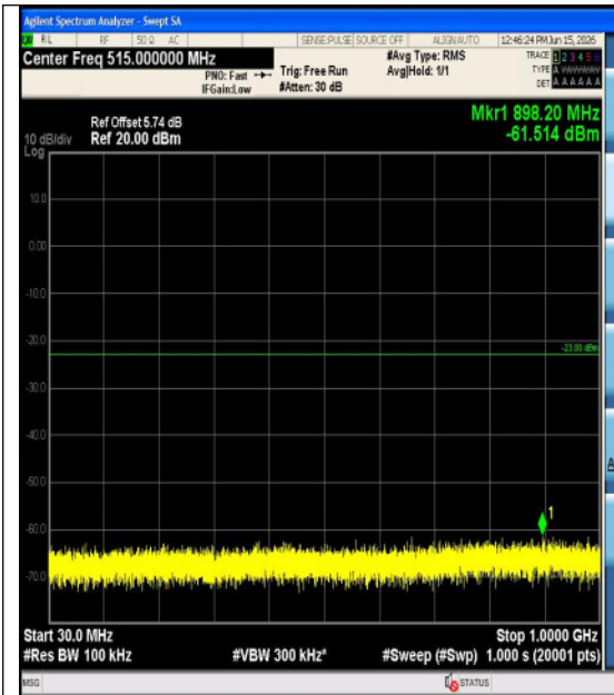
Band2-3MHz-QPSK-18900-15RB#0-3000~2000 0-PASS
