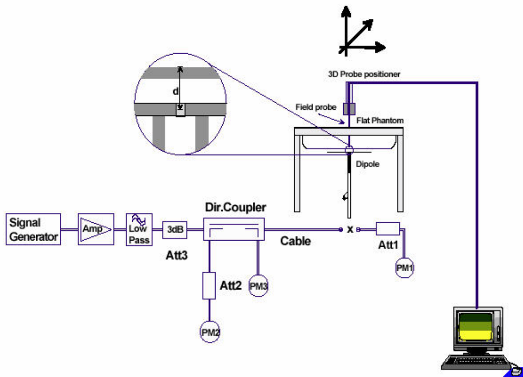
Picture 1 System Performance Check setup
